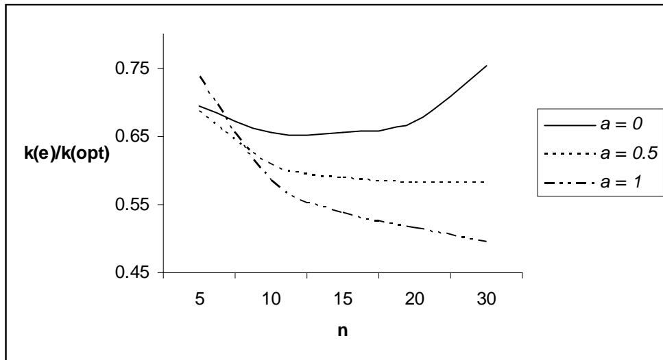
Figure 3: RJV equilibrium size relative to optimal size ( k^e/k^{opt} )
